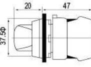
短柄带灯旋钮 Short shank with lamp knob
