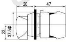
长柄带灯旋钮 Long handle with lamp knob
