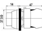
平头带灯按钮 Flat ribbon lamp button
