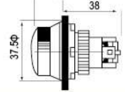
指示灯 Indicating lamp
