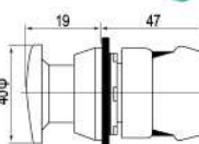
急停按钮 Emergency stop button
